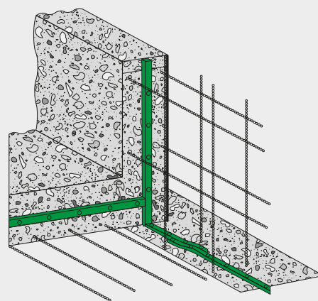
CONSTRUCTIONS JOINTS
